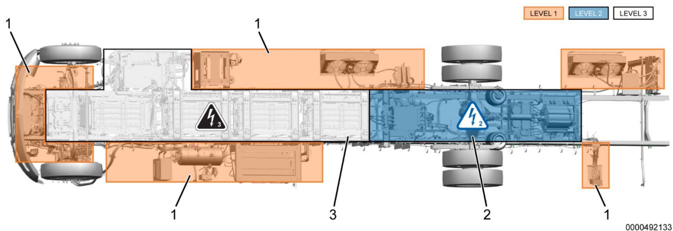
Figure 13. High-Voltage Isolation Levels / Zones (9-Battery Configuration, Viewed from Bottom)
