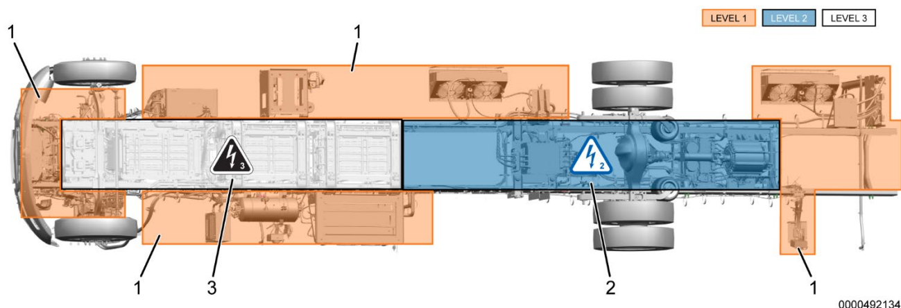
Figure 12. High-Voltage Isolation Levels / Zones (6-Battery Configuration, Viewed from Bottom)
