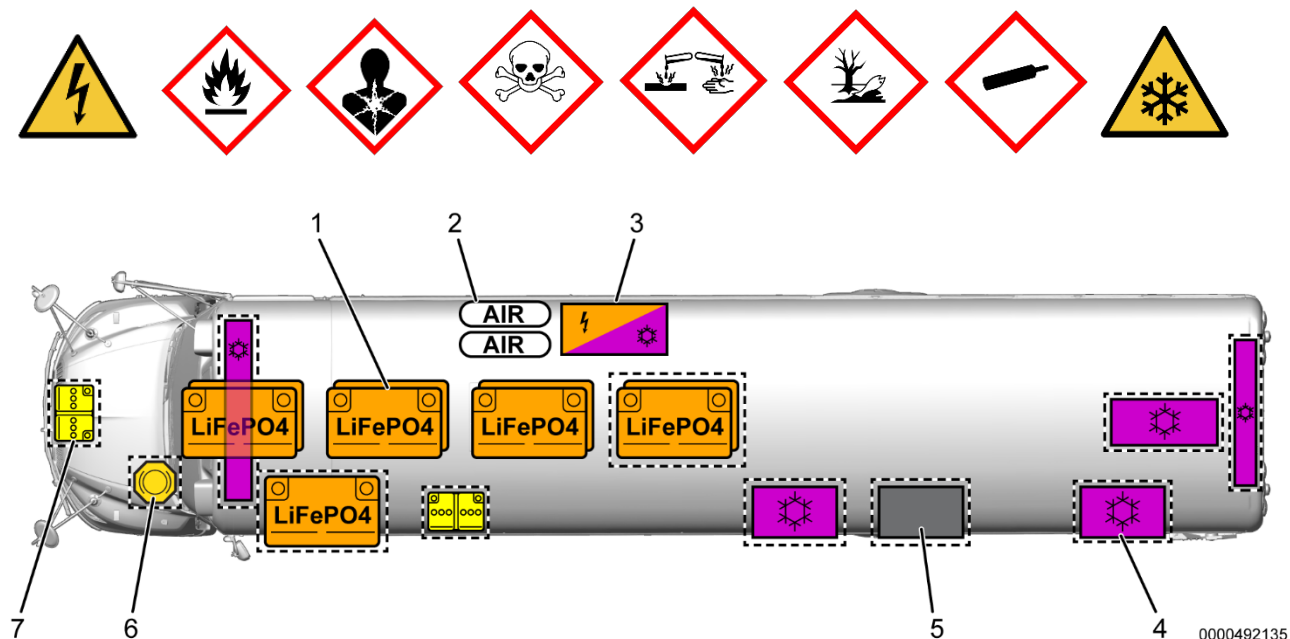
Figure 29. Stored Energy, Liquids, and Gases
