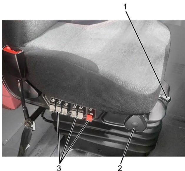
Figure 27. Driver Seat Controls
